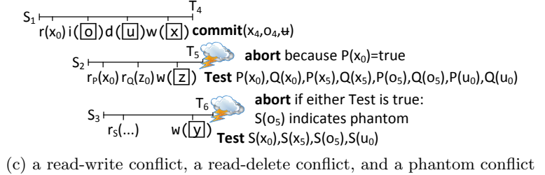
Figure 6: Example schedules in our MVCC model
